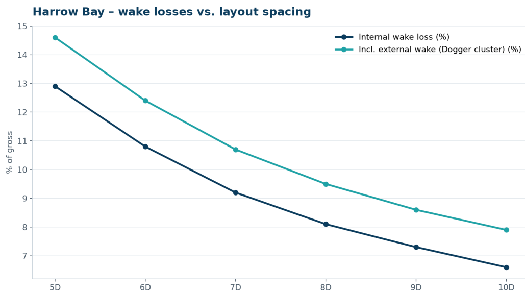
Figure 2 – Sensitivity of wake losses to turbine spacing (rotor diameters D = 236 m)
